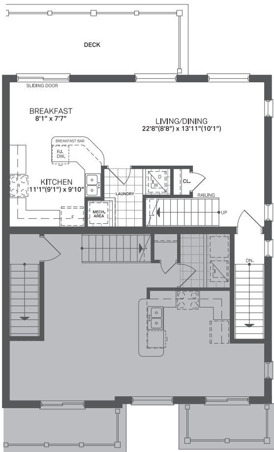
SECOND FLOOR
