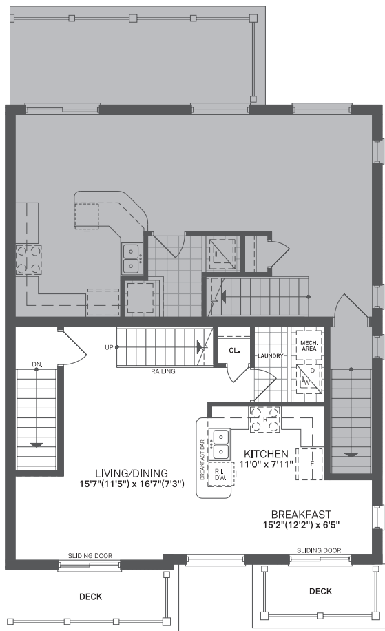
SECOND FLOOR
